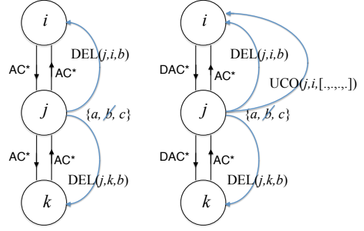
Figure 4. Three agents i, j, k in the same branch of the DFS tree. (Left) Maintaining AC*: Cost functions are AC* in both senses; deleting value b in D_j causes to send two DEL messages to i and k to restore AC*. (Right) Maintaining FDAC*: Cost functions are FDAC* (DAC* in one sense and AC* in the other); deleting value b in D_j causes to send two DEL messages to i and k to restore AC*, plus one UCO message to the higher agent i to restore DAC*.
