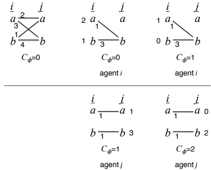
Figure 2. (UP) Left: Simple example with two agents i and j and two values per variable. Center: i projects C_{ij} on its unary costs. Right: i projects unary costs on C_\phi . (DOWN) Center: j projects C_{ij} on its unary costs, without considering previous projection of i (this is incorrect). Right: j projects unary costs on C_\phi , causing an incorrect increment.
